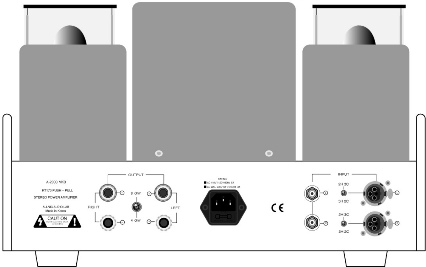
Figure 4: A-2000 MK3 Rear View
